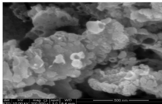
Fig. 6: Scanning Electron Microscopy Image showing PE- \text{Fe}_2\text{O}_3 NPs.
