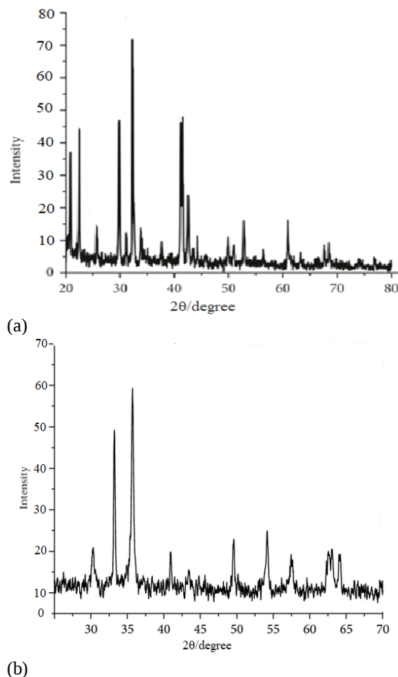
Fig. 5: The XRD analysis of (a) PE - \text{Fe}_2\text{O}_3 -NPs & (b) \text{Fe}_2\text{O}_3 NPs.
